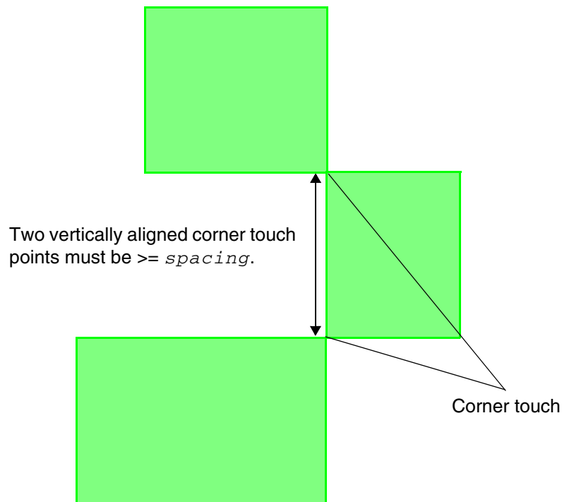
Illustration of CORNERSPACING spacing ALIGNEDONLY
