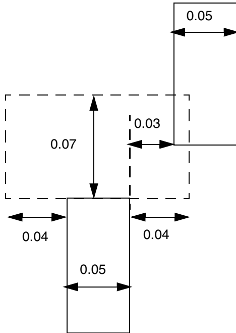
Figure 5-121 Example of Spacing Rule with EXACTWIDTH
