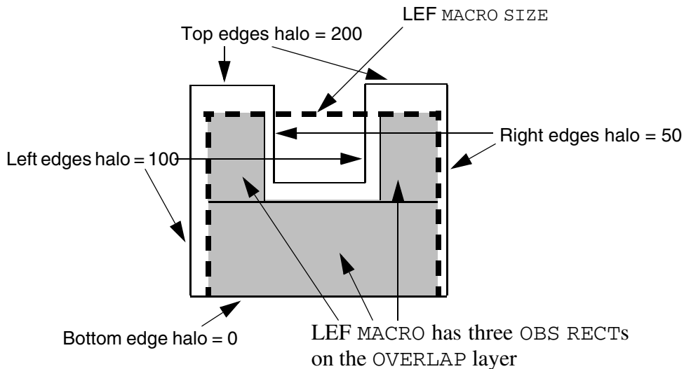
Figure 6-1 Component Halo
