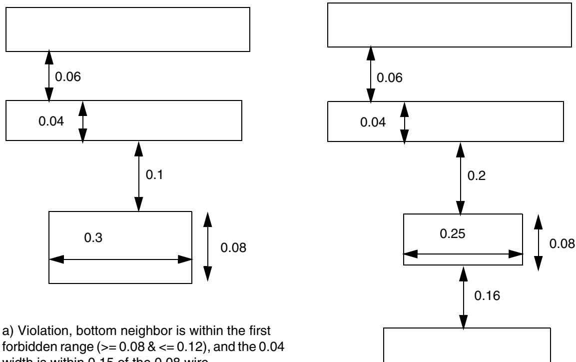
Figure 5-70 Illustration of FORBIDDENSPACING with WITHIN
