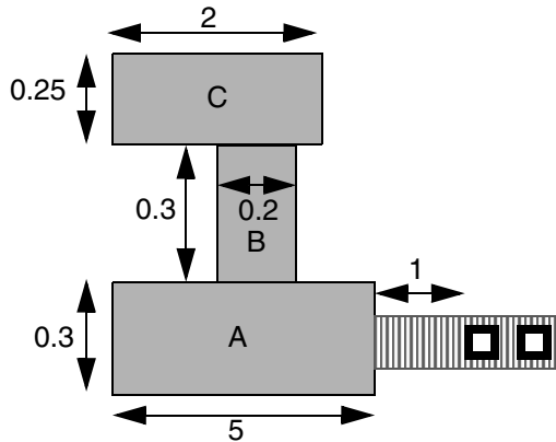
Figure 5-83 Minimum Cut Rule Example
