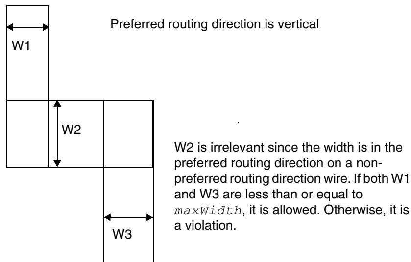
Figure 5-115 Illustration of Rectangle Only Rule
