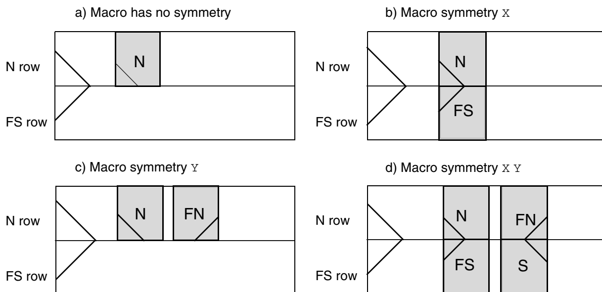
Figure 1-46 Legal Placements for Row Sites with Symmetry Y
