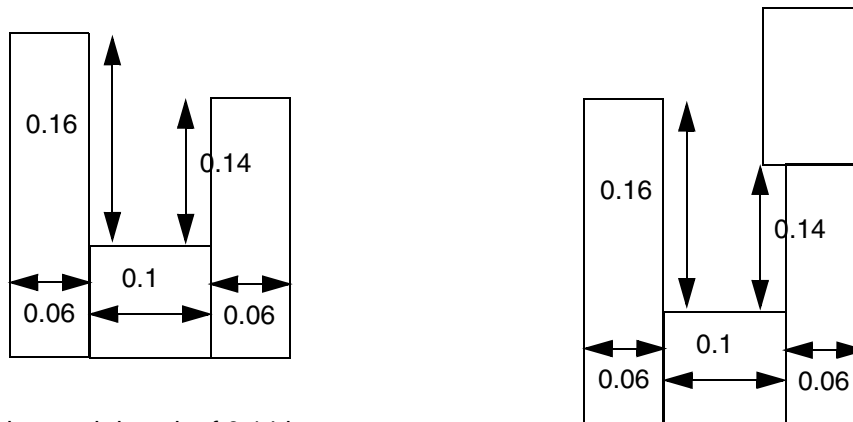
Figure 5-157 Illustration of Spacing Rule with NOTCHLENGTH and CONCAVEENDS
