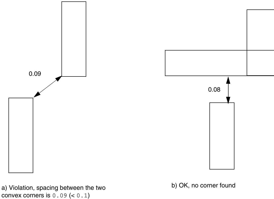
Figure 5-36 Illustration of Corner Spacing Rule with CORNERTOCORNER
