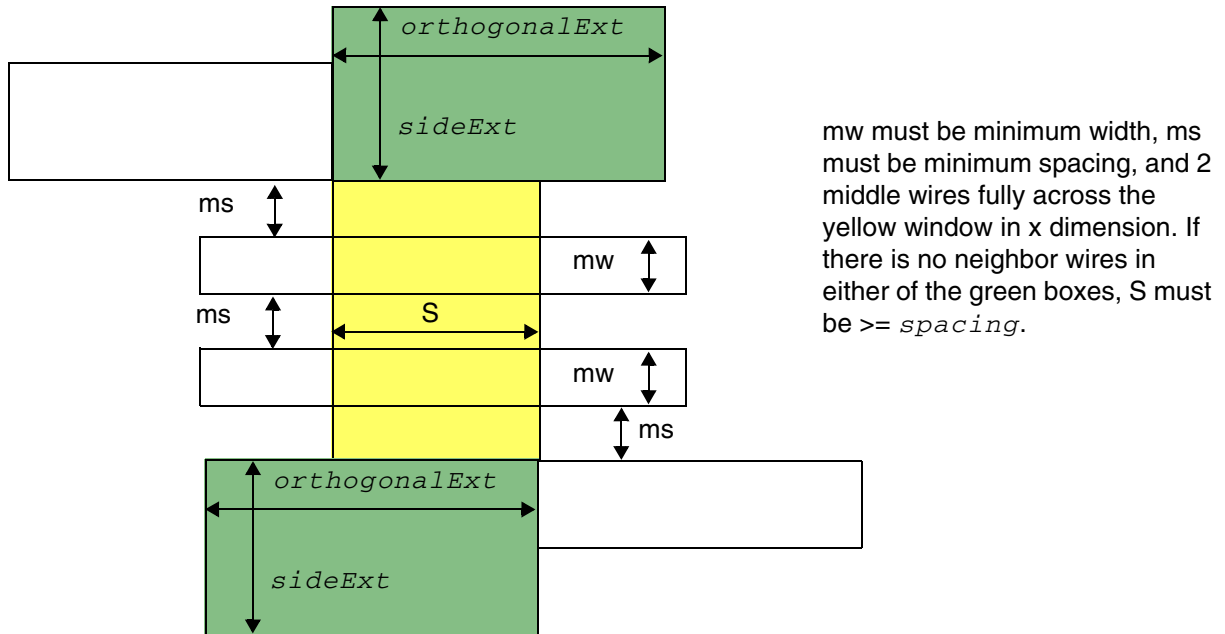
Figure 5-139 Illustration of Spacing Rule with CONVEXCORNERS
