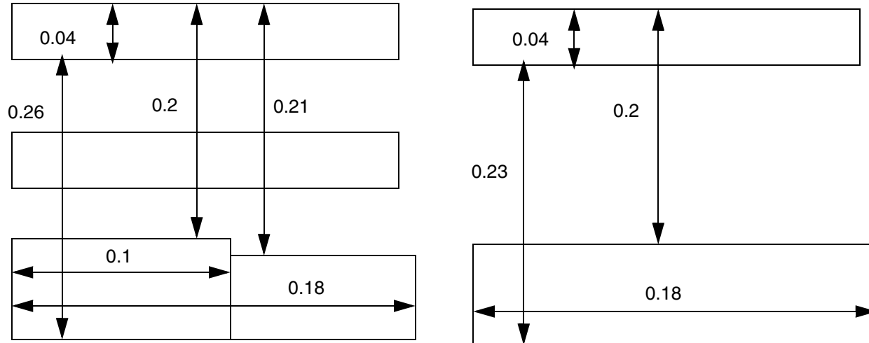
Figure 5-65 Illustration of FORBIDDENSPACING with WIDTH and PRL
