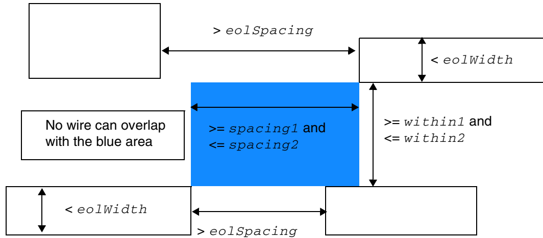
Figure 5-26 Illustration of the Corner EOL Keep-out Rule with SPACING
