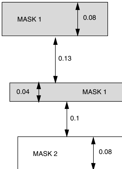
Figure 5-72 Illustration of FORBIDDENSPACING with WIDTHRANGE
