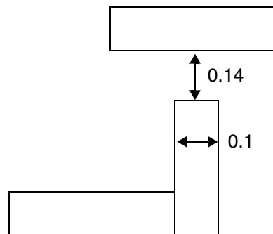
Figure 5-132 Example of EOL Spacing Rule with EQUALRECTWIDTH
