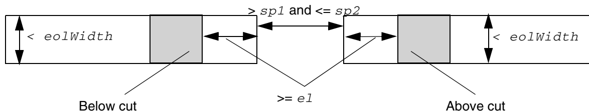
Figure 5-39 Illustrations of Enclosure with EOL Rule with ENCLOSURESPACING
