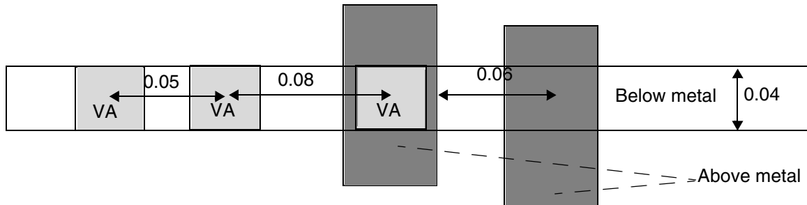
Figure 2-148 Illustration of the Same-Metal Aligned Cuts Rule with NOVIAMETALOVERLAP
