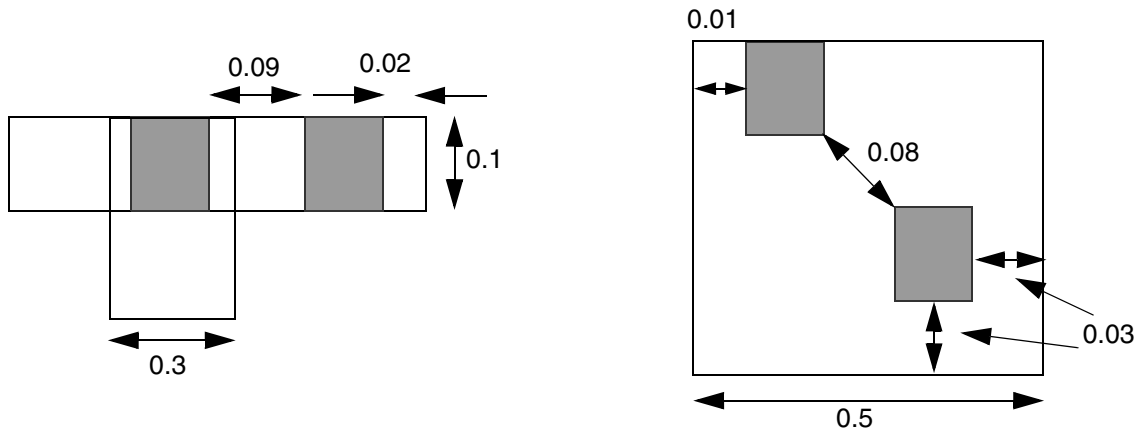
Figure 2-34 Illustrations of the Enclosure Rule With REDUNDANTCUT
