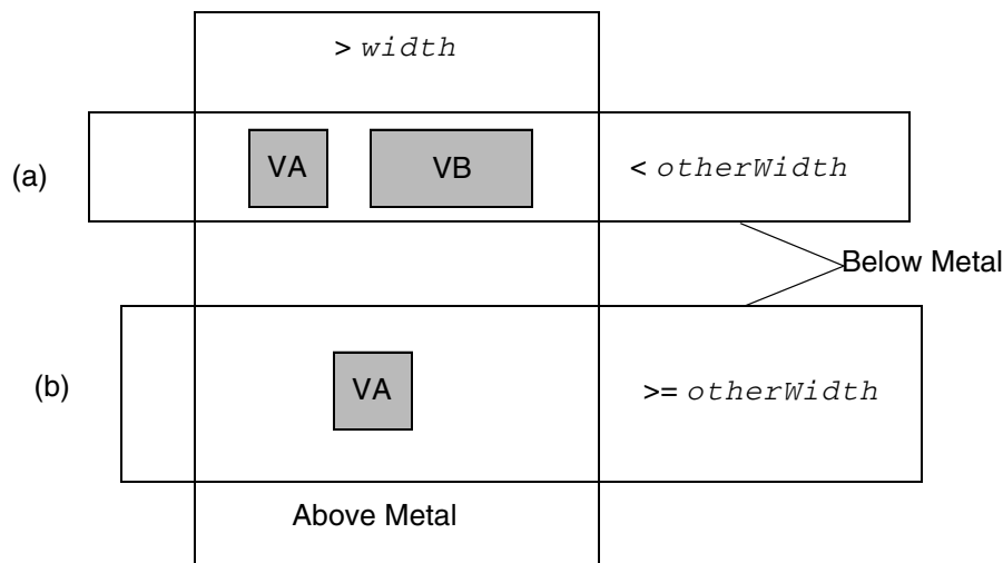
Figure 5-86 Illustration of Minimum Cut Rule with DIFFCUTCLASS and EXCEPTOTHERWIDTH
