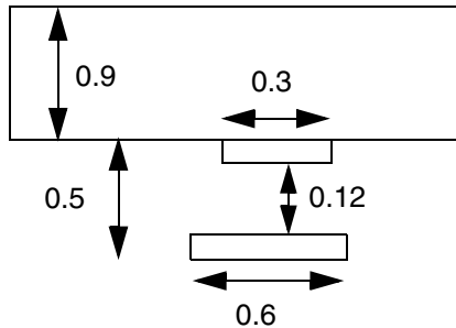
Figure 5-162 Illustration of Spacing Table with JOGTOJOGSPACING
