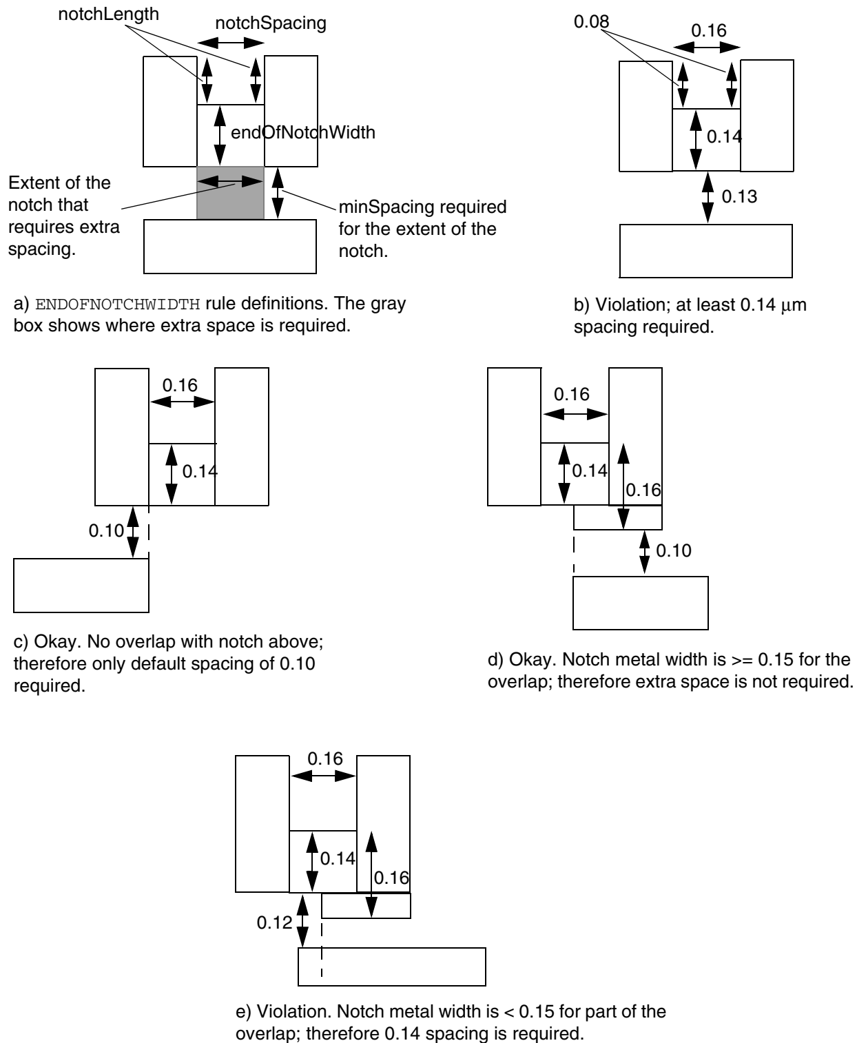
Figure 5-15 End Of Notch Width Rule Definitions
