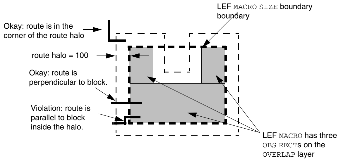
Figure 6-2 Route Halo
