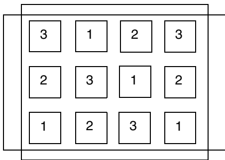
Via-master cut masks for VIA1_2.
