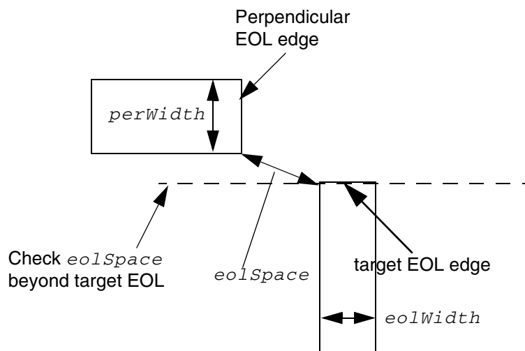
Figure 5-147 Illustration of Perpendicular EOL Spacing Parameters
