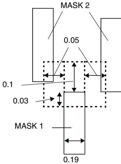
Figure 5-51 Illustration of EOL Keep Out Rule with Mask and Two Sides
