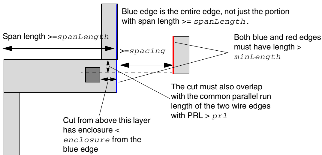
Figure 5-117 Illustration of SPANLENGTHENCLOSURESPACING
