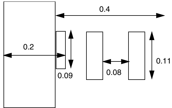
Figure 5-66 Illustration of FORBIDDENSPACING with WIDTH and WITHIN
