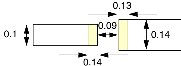
Figure 5-40 EOL Extension Spacing Rule Example
