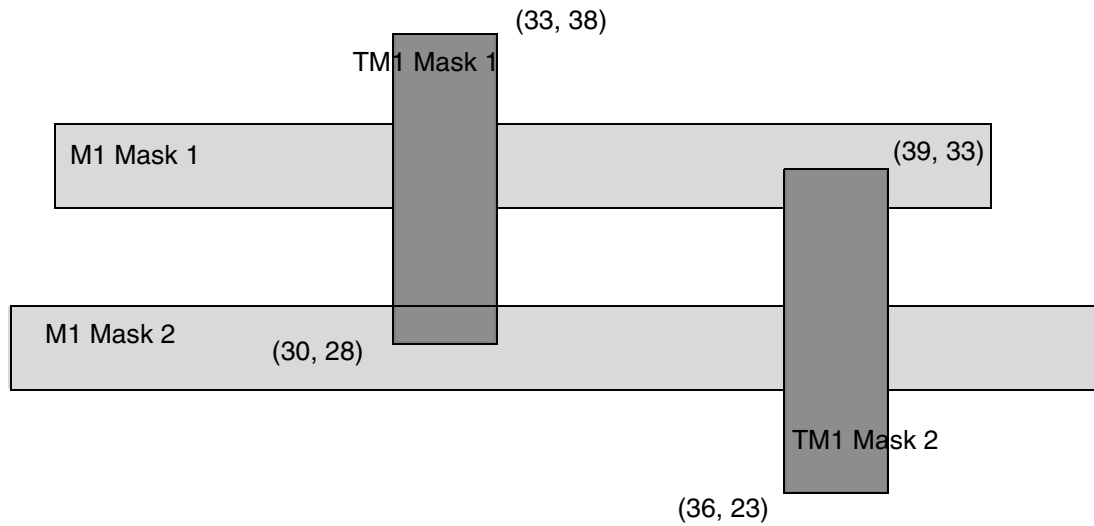
Figure 6-3 Trim Metal Layer Shapes in the FILLS Section
