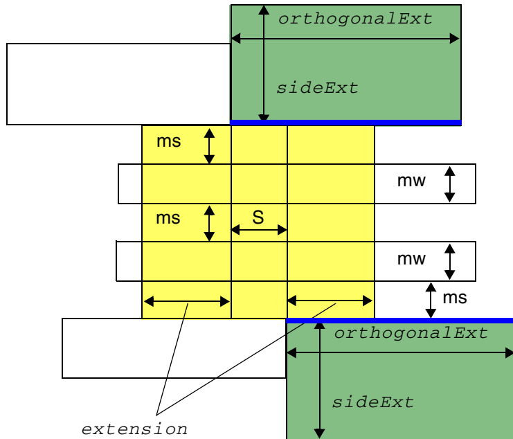
Figure 5-140 Illustration of Spacing Rule with CONVEXCORNERS
