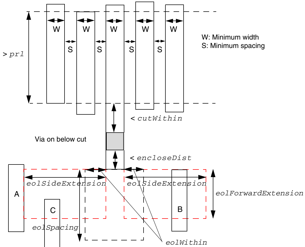
Figure 5-64 Illustration of FIVEWIRESEOLSPACING
