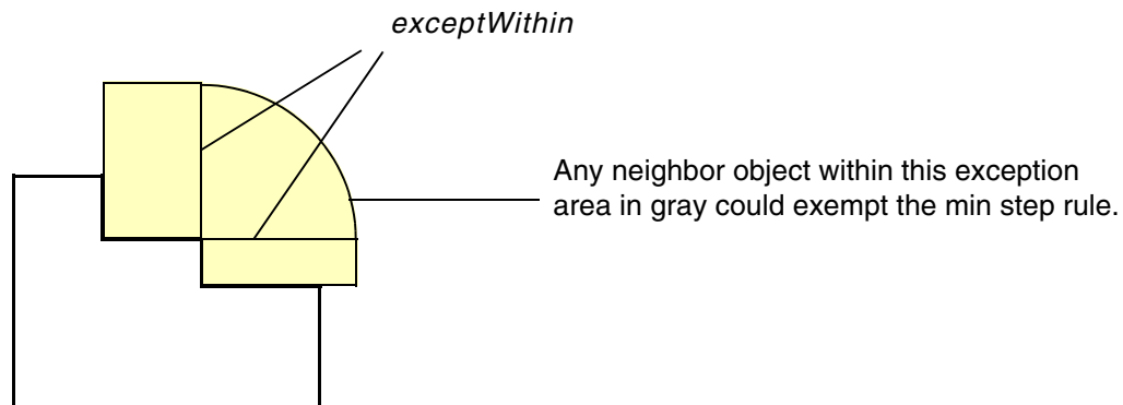
Figure 5-97 EXCEPTWITHIN exceptWithin in CONVEXCORNER in the MinStep Rule
