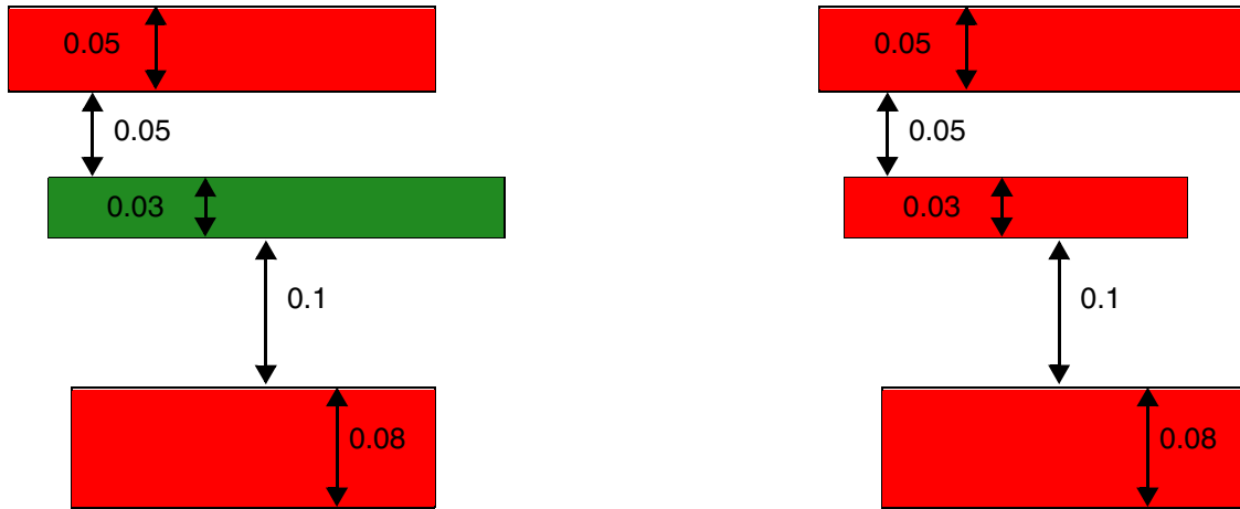
Figure 5-177 Illustration of TWOWIRESFORBIDDENSPACING
