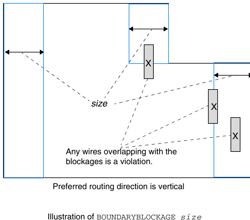
Figure 5-22 Illustration of the Boundary Blockage Rule
