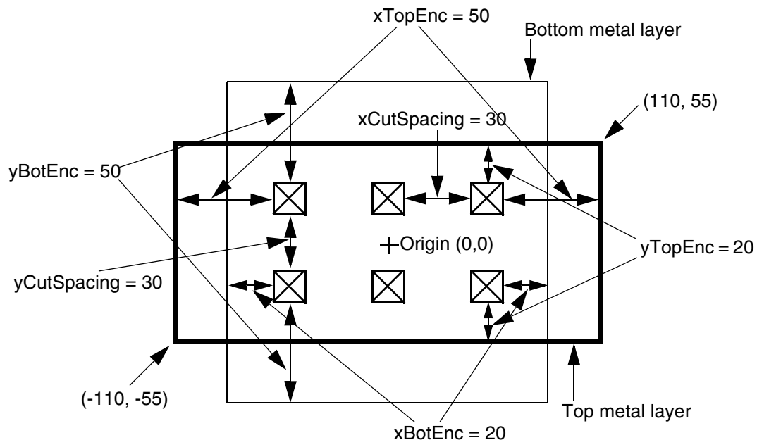
Figure 1-57 Via Rule
