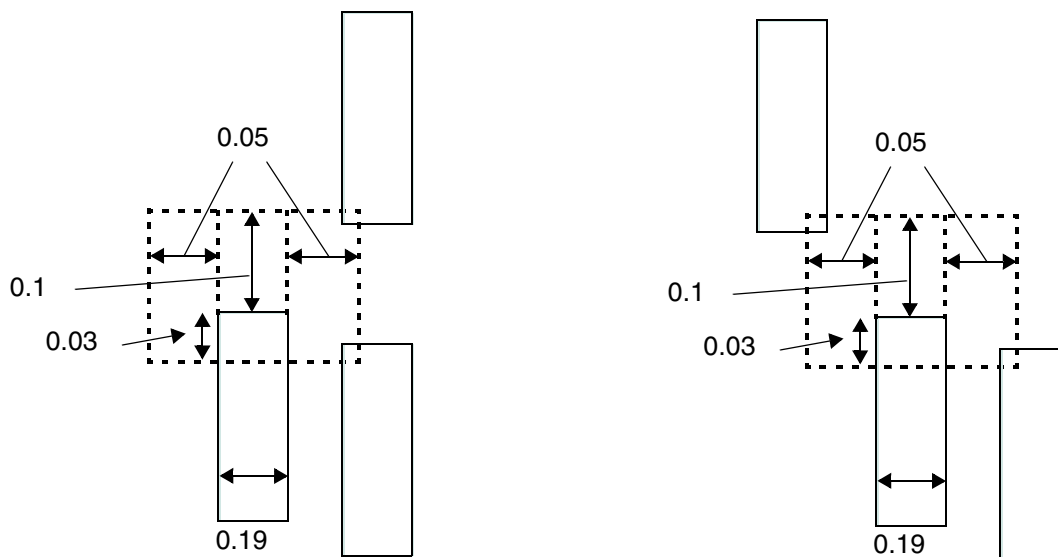
Figure 5-49 Illustration of EOL Keep Out Rule with FRONTEDGE and BACKEDGE
