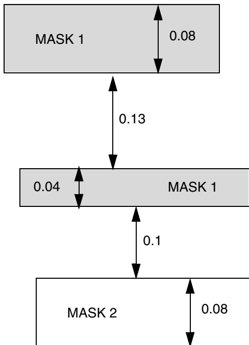
Figure 5-73 Illustration of FORBIDDENSPACING with WIDTHRANGE
