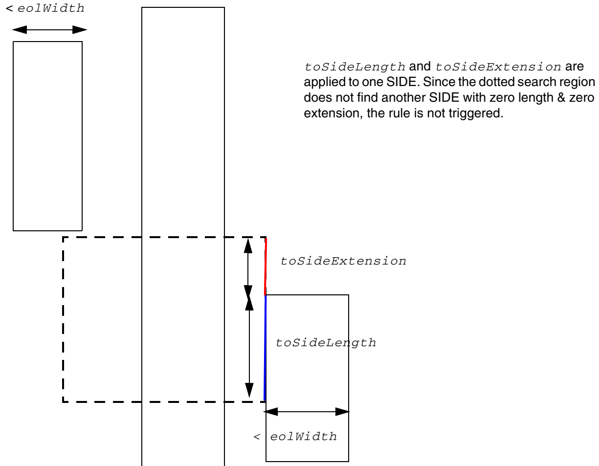
Figure 5-107 Illustration of SIDELENGTH in OPPOSITEEOLSPACING
