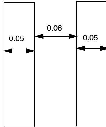
Figure 5-169 Illustration of Spacing Table Rule with DIRECTIONALSPANLENGTH
