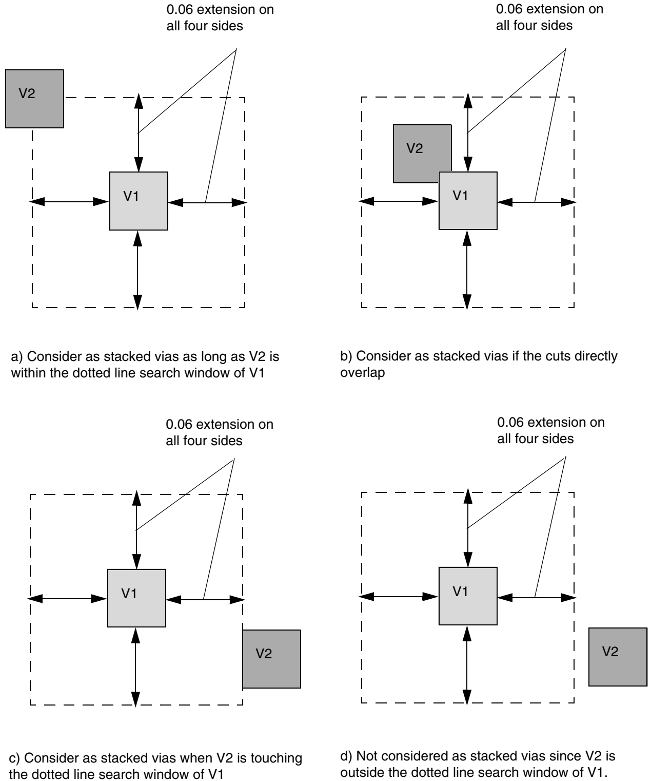
Figure 1-12 Illustration of Max Via Stack Rule with WITHIN LOWCUTSIZE
