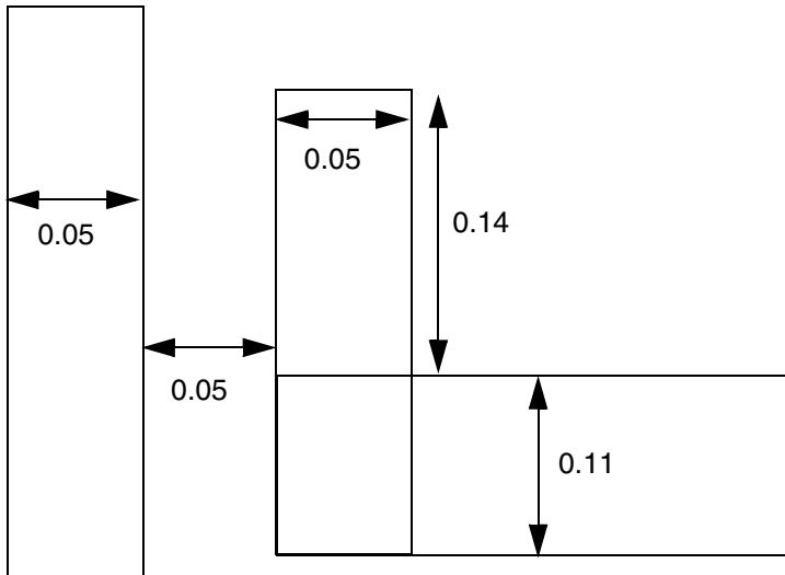
Figure 5-176 Illustration of PARALLELRUNLENGTH with WRONGDIRECTION
