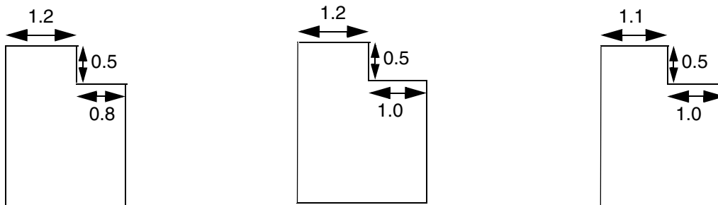
Figure 5-94 MinStep Rule with MINADJACENTLENGTH
