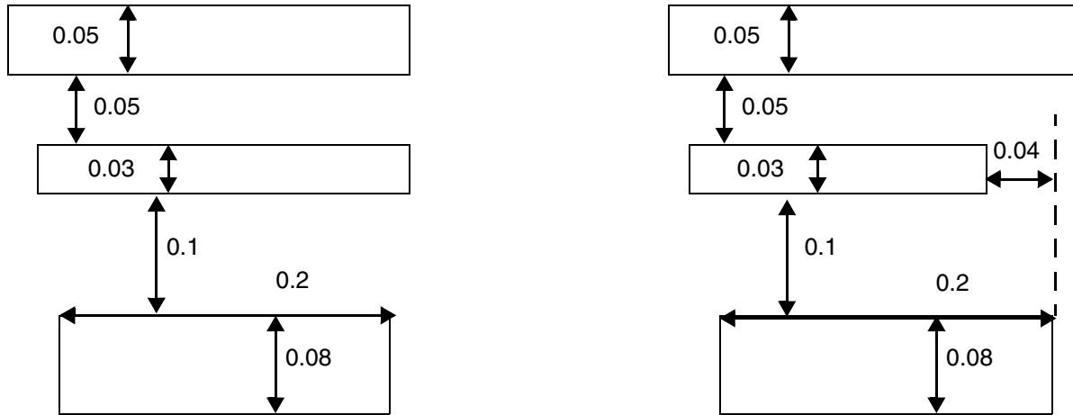
Figure 5-179 Illustration of TWOWIRESFORBIDDENSPACING with IGNOREMIDDLE
