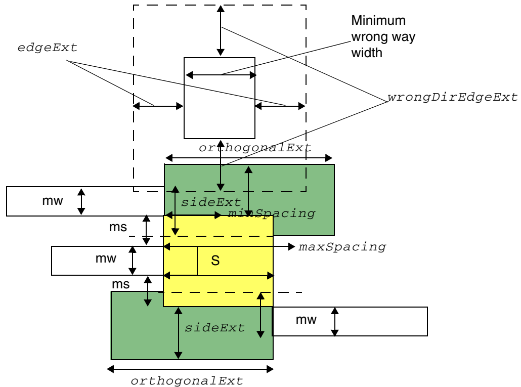
Figure 5-145 Illustration of Spacing Rule with EXCEPTWRONGDIRWIRE in CONVEXCORNERS
