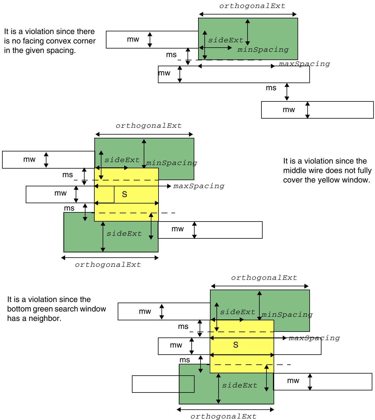
Figure 5-144 Illustrations of Spacing Rule with REVERSE in CONVEXCORNERS
