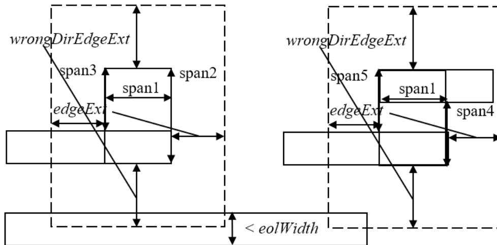
Figure 5-183 Illustration of WRONGDIRECTIONEOLEKEEPOUT Rule
