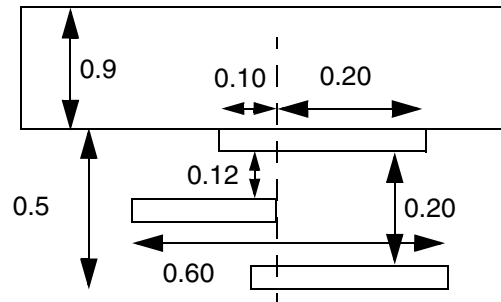
Figure 5-164 Illustration of Spacing Table with JOGTOJOGSPACING
