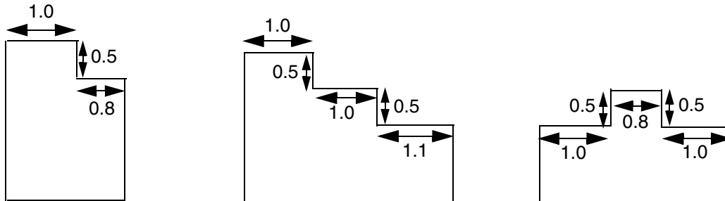
Figure 5-93 MinStep Rule with Adjacent Edge
