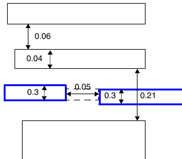
Figure 5-74 Illustration of FORBIDDENSPACING with EXCEPTWIREWIDTHSPACING
