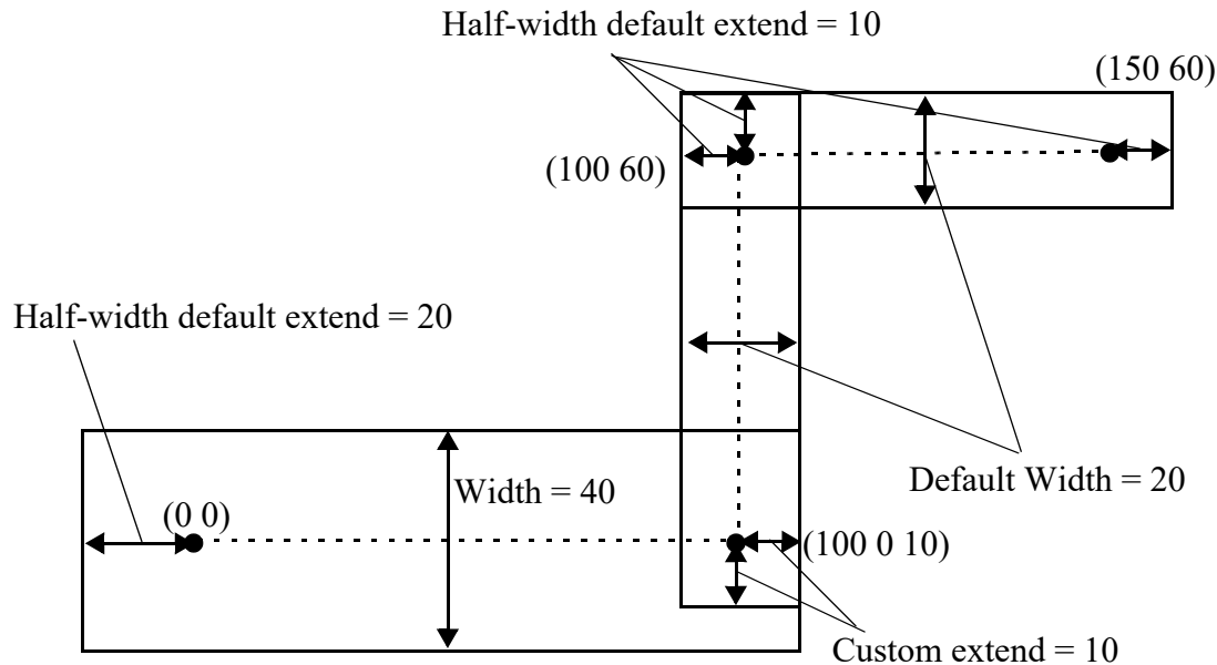
Figure 6-6 Routing Points - Usage of Width
