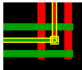
d) -shield_enclose_vias true Adds shields all around vias in the preferred direction.
