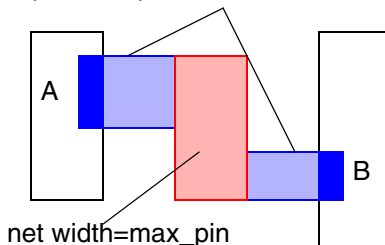
c) set_taper_width_nets -taper_style to_first_via -net_width max_pin
